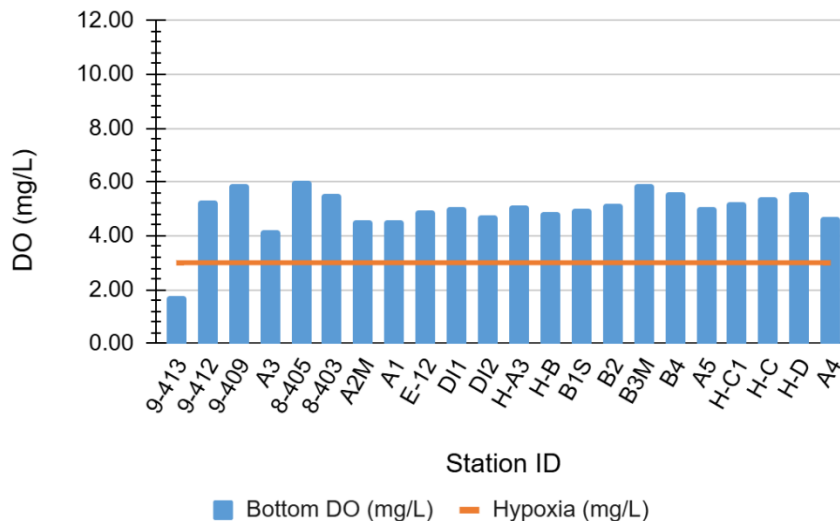
WLIS Bottom Dissolved Oxygen, Survey #12 09/10/26
