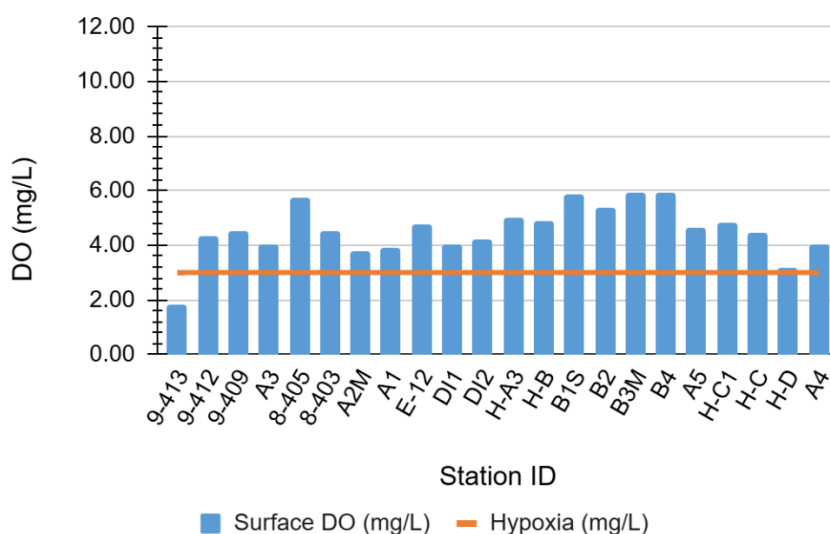
WLIS Surface Dissolved Oxygen, Survey #11 09/01/26
