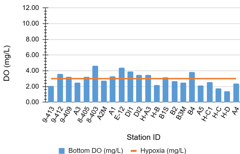
WLIS Bottom Dissolved Oxygen, Survey #11 09/01/26
