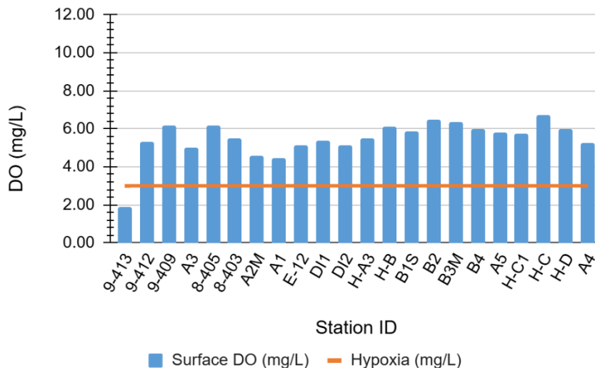
WLIS Surface Dissolved Oxygen, Survey #12 09/10/26
