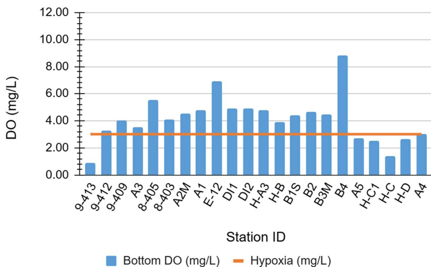
WLIS Bottom Dissolved Oxygen, Survey #2 07/01/26
