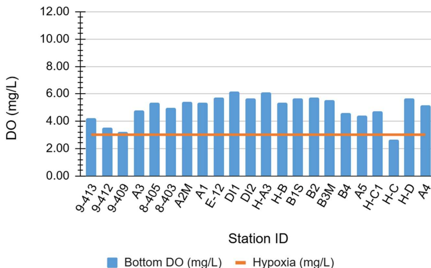
WLIS Bottom Dissolved Oxygen, Survey #1 06/24/26
