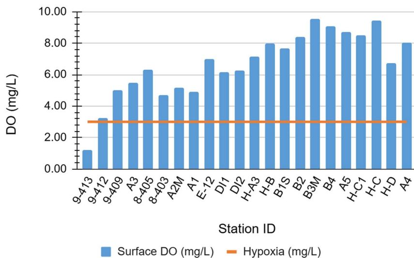
WLIS Surface Dissolved Oxygen, Survey #2 07/01/26
