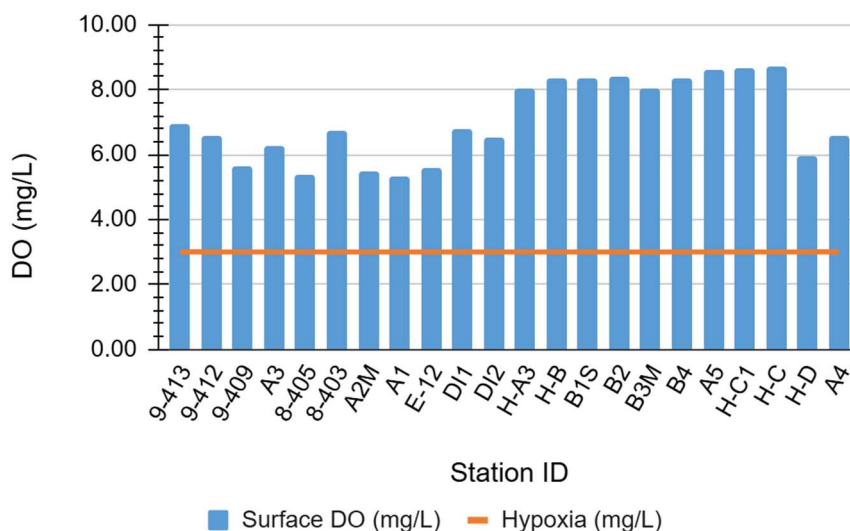
WLIS Surface Dissolved Oxygen, Survey #1 06/24/26
