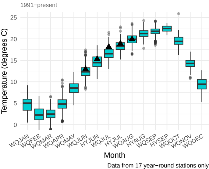
Average Bottom Water Temperatures
