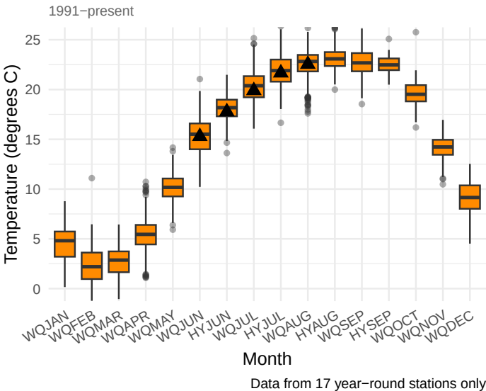
Average Surface Water Temperatures
