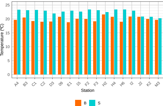
Temperature Across Long Island Sound WQAUG26
