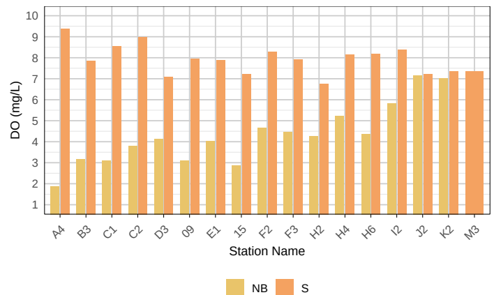
Dissolved Oxygen Concentrations Across the Long Island Sound WQAUG26
