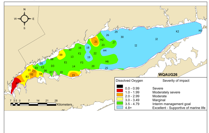
Dissolved Oxygen Concentrations Across the Long Island Sound WQAUG26
