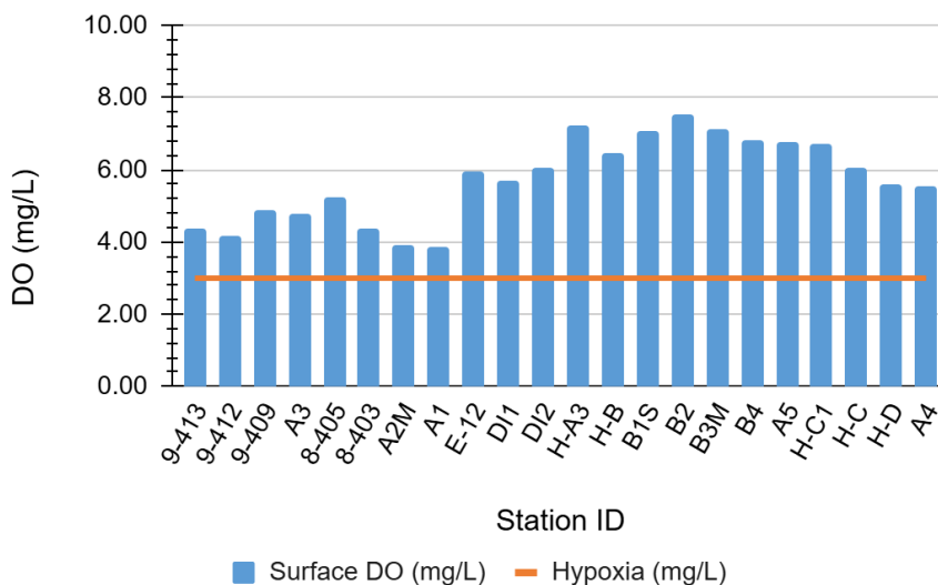
WLIS Surface Dissolved Oxygen, Survey #6 07/30/24
