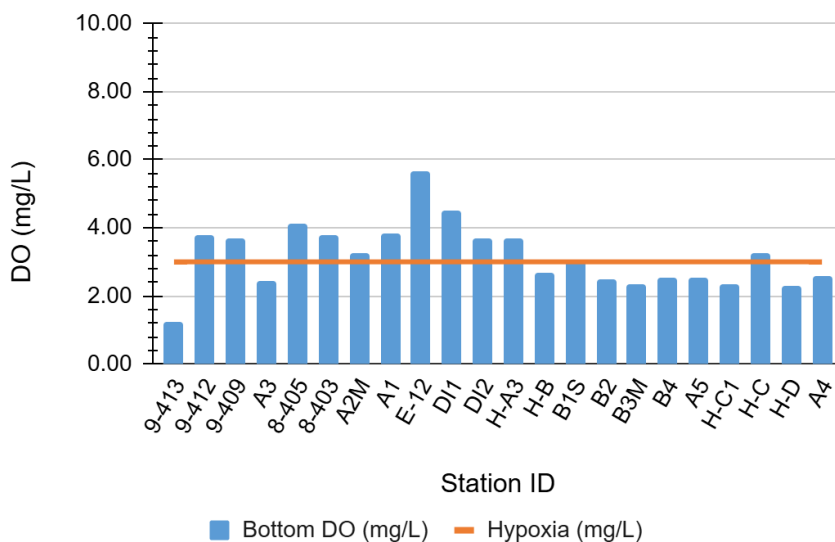
WLIS Bottom Dissolved Oxygen, Survey #6 07/30/24
