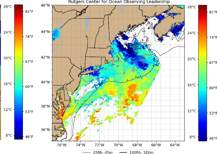
NOAA-18 Sea Surface Temperature: June 13 2023 1635 GMT Rutgers Center for Ocean Observing Leadership
