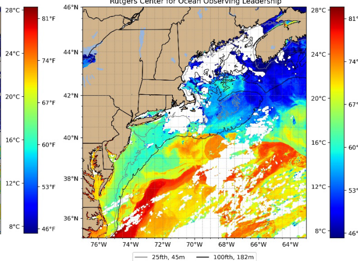
NOAA-18 Sea Surface Temperature: June 09 2023 1543 GMT Rutgers Center for Ocean Observing Leadership
